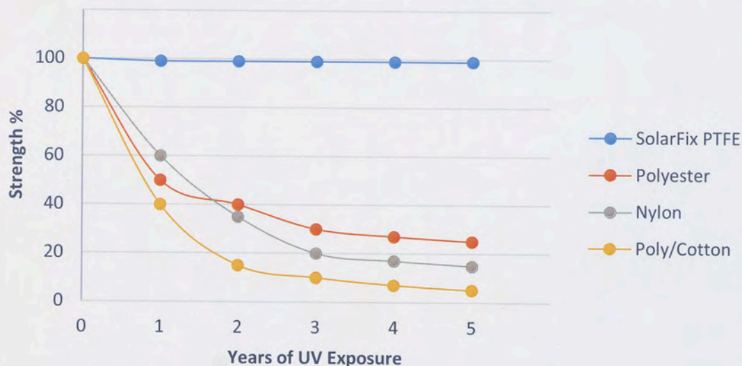
Strength Comparison After UV Exposure
